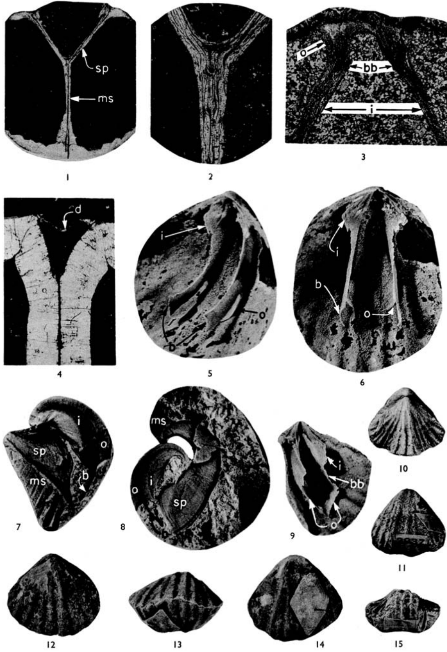
AMSDEN, Pentameridae
