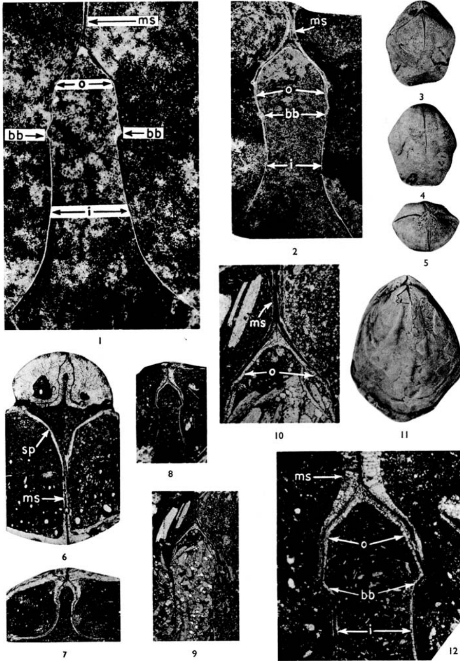
AMSDEN, Pentameridae
