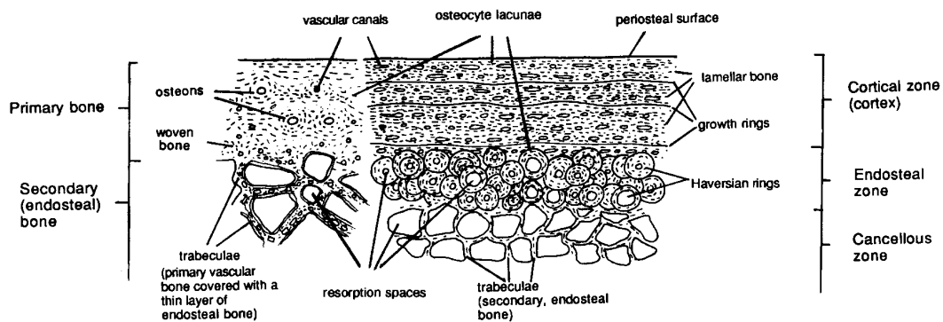
TEXT-FIG. 1. Sketch explaining general histological terminology of a transverse section through a normal fossil vertebrate bone. Not to scale.
