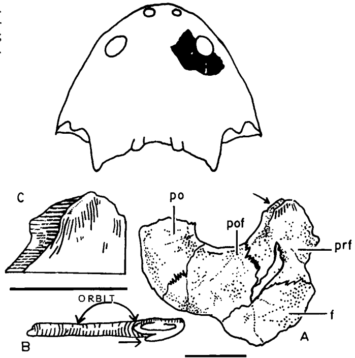
TEXT-FIG. 6. Compsoceros cosgriffi gen. et sp. nov., ISI A 35. Prefrontal prominence in A, ventral view; B, lateral view; C, enlarged. Scale bars represent 50 mm.
