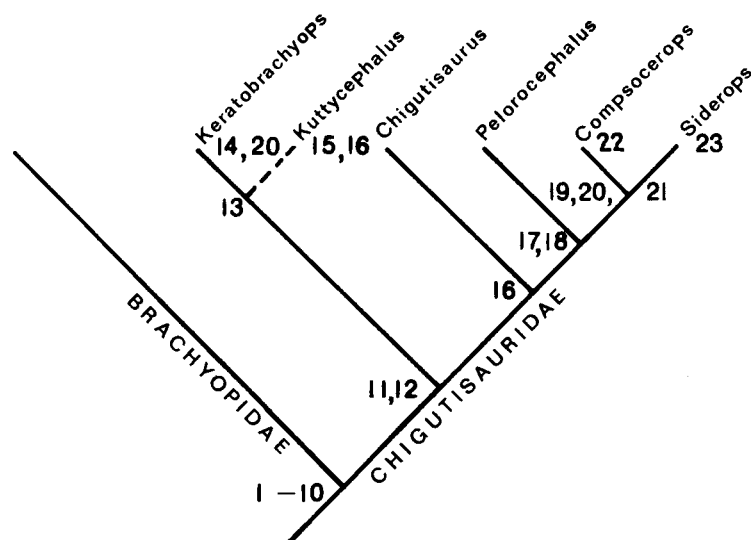
TEXT-FIG. 19. Cladogram depicting relationships of chigutisaurids. Characters used are listed in Table 2.
