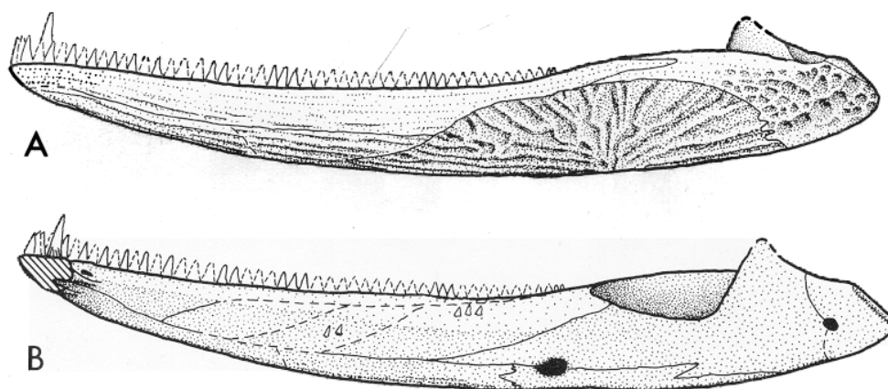
TEXT-FIG. 5. Parotosuchus aliciae sp. nov., restoration of mandible (oriented parasagittally) based on holotype and paratype specimens. A, labial view; B, lingual view. \times 4 natural size.
