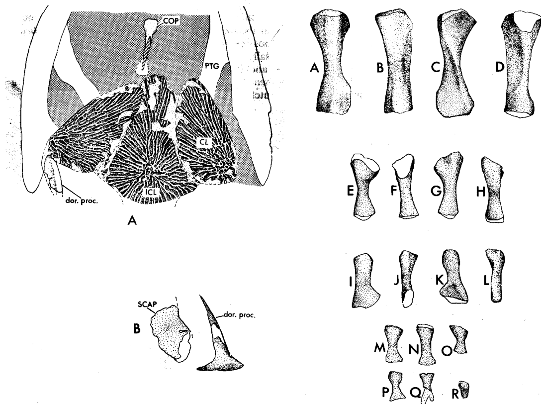
TEXT-FIG. 6. (left). Parotosuchus aliciae sp. nov., pectoral girdle and hyoid elements as preserved. \times 2 natural size. A, clavicles, interclavicle, and copula of holotype, QM F12281, based on polyester resin cast; B, lateral view of right partial clavicle and scapulocoracoid of paratype, QM F12282. Abbreviations: CL, clavicle; COP, copula; dor.proc., dorsal process of clavicle; ICL, interclavicle; SCAP, scapula; remainder as in text-fig. 2.
