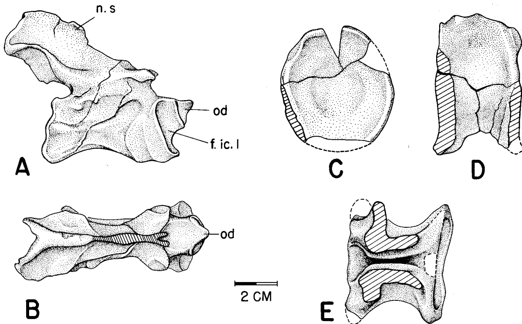
TEXT-FIG. 1. Cf. Staurikosaurus sp., MCZ 7064. A, B, atlas centrum, atlas intercentrum, and axis, in A, right lateral and B, dorsal view. C-E, centrum of a posterior dorsal vertebra, in C, anterior, D, lateral, and E, dorsal view. Abbreviations: f.ic.l—facet for atlas intercentrum, n.s—neural spine of axis, od—odontoid process.
