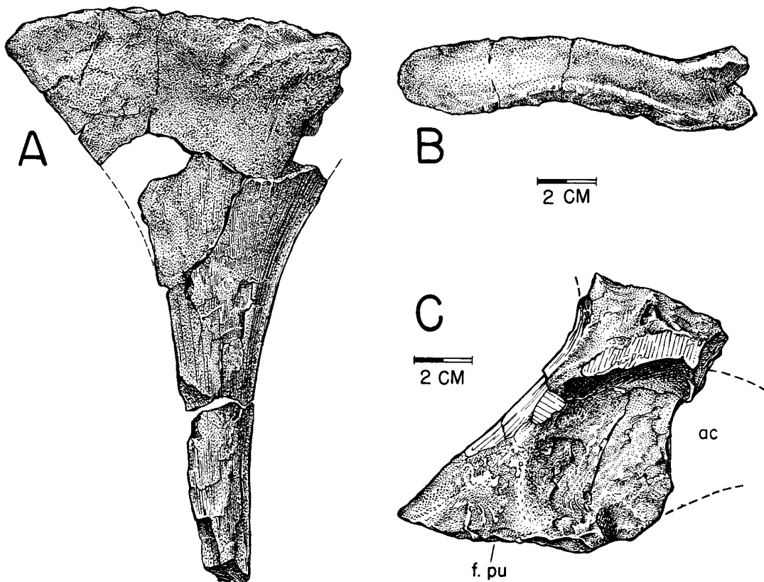
TEXT-FIG. 4. Cf. Staurikosaurus sp., MCZ 7064. A, B, partial right ischium in A, lateral and B, proximal end view. C, partial left ilium in lateral view. Abbreviations: ac—acetabular wall, f.pu—articular facet for pubis.
