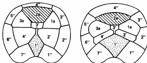
TEXT-FIG. 18. (left) Epithecal tabulation of Proto-peridinium (Proto-peridinium) conicoides (Paulsen) Balech (after Wall and Dale 1968).
