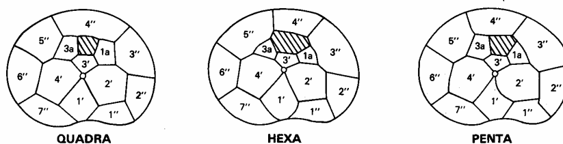
TEXT-FIG. 2. Examples of the three different styles of dorsal epithecal tabulation (after Graham 1942). The second dorsal intercalary plate is hachured.
