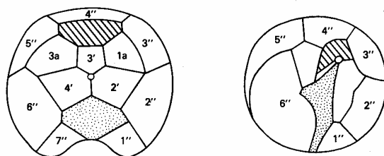
TEXT-FIG. 3 (left). Epithecal tabulation of Protoperidinium ( Protoperidinium ) pellucidum Bergh ex Loeblich, Jr. and Loeblich, III (after Lebour 1925).
