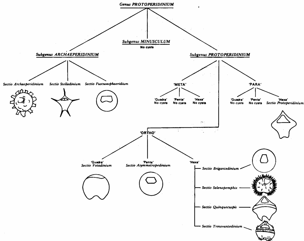
TEXT-FIG. 24. Recent and Quaternary Protoperidinium cyst types and their respective positions in the taxonomic subdivision of the genus.
