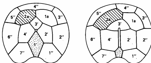
TEXT-FIG. 5 (left). Epithecal tabulation of Protoperidinium ( Archaeperidinium ) minutum (Kofoid) Loeblich, III (after Wall and Dale 1968).
