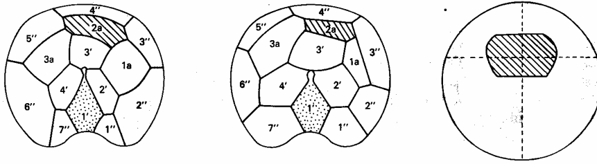
TEXT-FIG. 15 (left). Epithecal tabulation of a hexa Protoperidinium ( Protoperidinium ) punctulatum (Paulsen) Balech (after Wall and Dale 1968).
