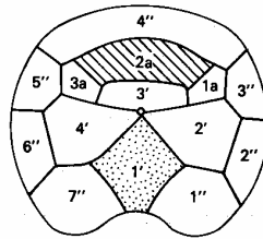
TEXT-FIG. 14. Epithecal tabulation of Protoperidinium ( Protoperidinium ) oblongum (Aurivillius) Balech (after Wall and Dale 1968).
