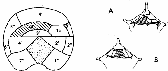
TEXT-FIG. 8 (left). Epithecal tabulation of Proto-peridinium (Archaeperidinium) compressum (Abé) Balech (after Wall and Dale 1968).
