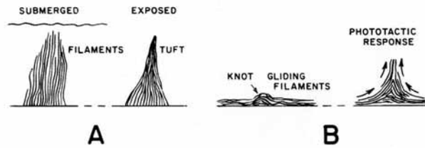
TEXT-FIG. 2. Mechanisms of tuft formation. A. Tufts caused by exposure of filaments (after Horodyski 1977, fig. 3r). B. Tufts formed by filaments gliding upwards over a knot (after Walter et al. 1976, fig. 36.3).
