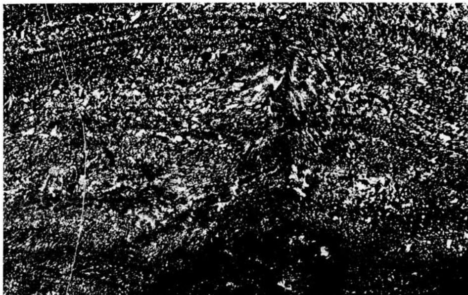
TEXT-FIG. 1. Detail of structure. Light areas are calcite filled voids. Photograph from thin section X7. Specimen from Huish Colliery Quarry (ST 696543, see Savage 1977). (University of Reading, Dept. of Geology, Archive No. S26675).
