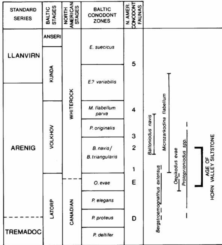
TEXT-FIG. 6. Correlation of the Horn Valley Siltstone with the European and the North American succession.
