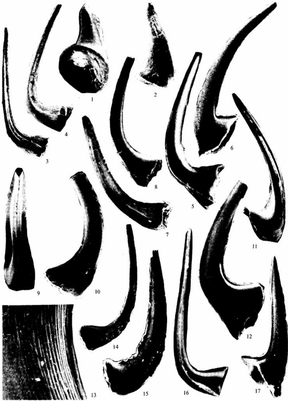
COOPER, Ordovician conodonts
