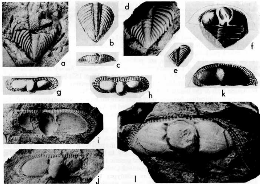
TEXT-FIG. 1. a-e , Celtencrinurus multisegmentatus (Portlock). a , GSM 35416, pygidium, \times 2 . b , c , reproductions of Portlock's figures of the same specimen (1843, pl. 3, fig. 6 a , b ), \times 1 . d , GSM 35417, lectotype, pygidium, \times 2 . e , reproduction of Portlock's figure of the same specimen (1837, pl. 2, fig. 7), \times 1 . f-l , Cryptolithus latus Portlock. f , reproduction of Portlock's figure of a specimen not now known (1837, pl. 2, fig. 8), \times 1 . g , h , reproductions of Portlock's 1843 pl. 1 B , figs. 11, 12 respectively, \times 1 . i , GSM 14016, cephalon, the supposed original of Portlock's 1843 figures, \times 2 . j , latex cast from GSM 14016, \times 2 . k , reproduction of Portlock's 1837 pl. 1, fig. 5, \times 1 . l , GSM 14019, lectotype, cephalon, the original of Portlock's 1837 figure, \times 2 . All specimens are from the Killey Bridge Formation (Ashgill Series, Cautleyan Stage), Pomeroy district, Co. Tyrone.
