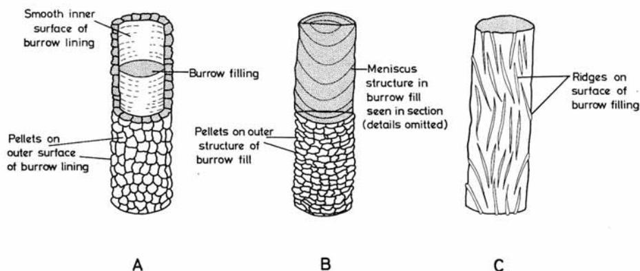
TEXT-FIG. 1. Diagram of types of Ophiomorpha occurring in the Weald Clay sandstones. Sectioned parts are stippled. \times 1 approx. A, Type 1, agreeing with the typical form of O. nodosa . B, Type 2, with meniscus fill (detailed structure of fill omitted). C, Type 3, comparable to Halymenites striatus .
